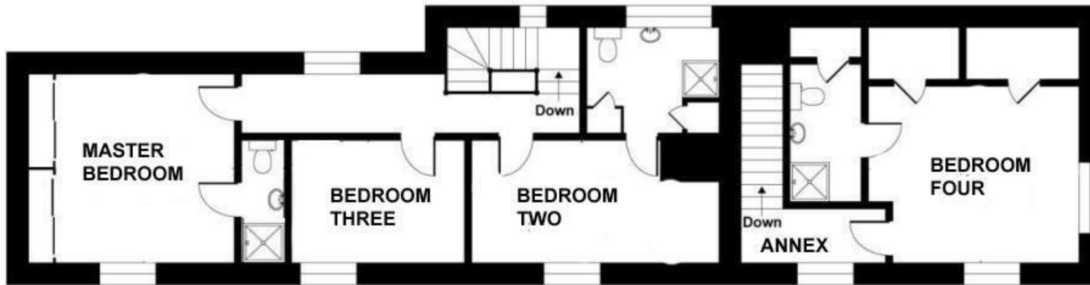
FIRST FLOOR
